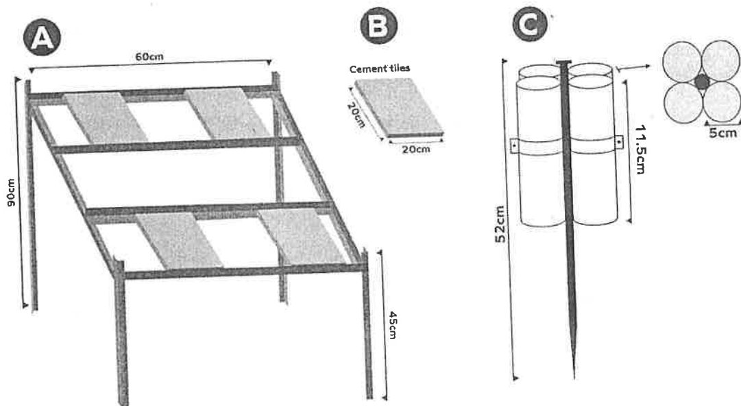
Figure 1: Dimension details of settlement panel (a) with tiles (b) and sedimentation trap (c)
