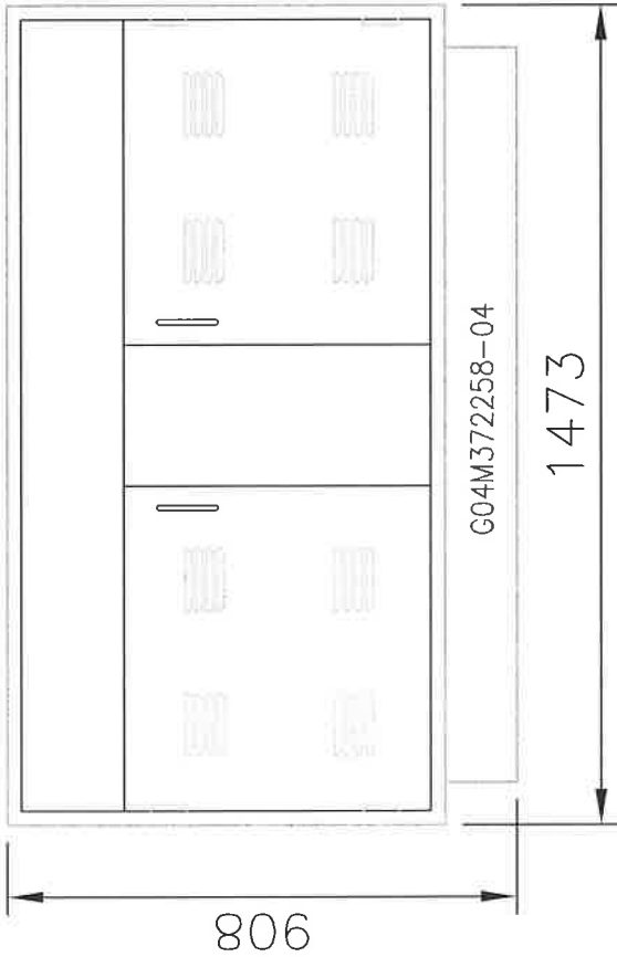
Elevation View
